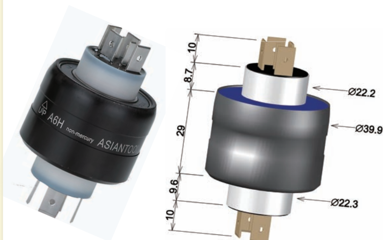
A6H NM (non-mercury) 4poles/30A & 2poles/4A AC250V
