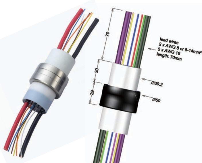
21005W 2poles/80-150A/AC250V 5poles/4-10A/AC250V
