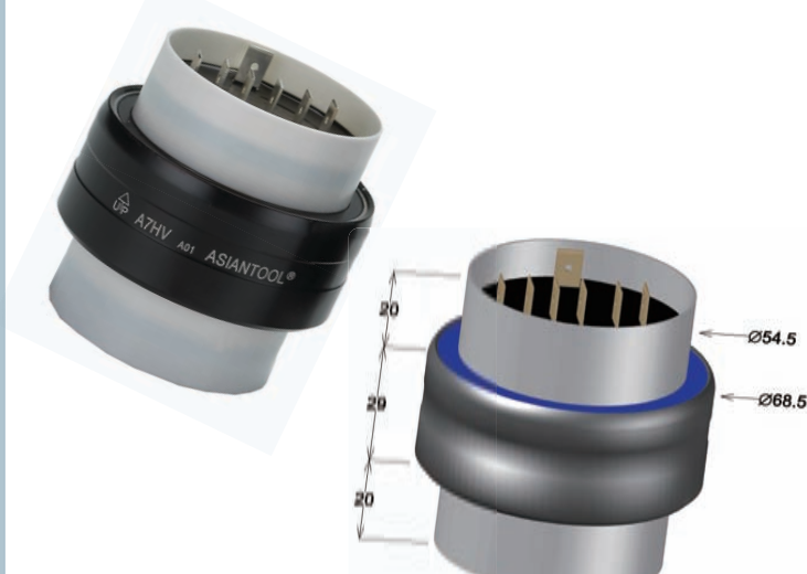
A7HV 7poles/30A/AC500V
