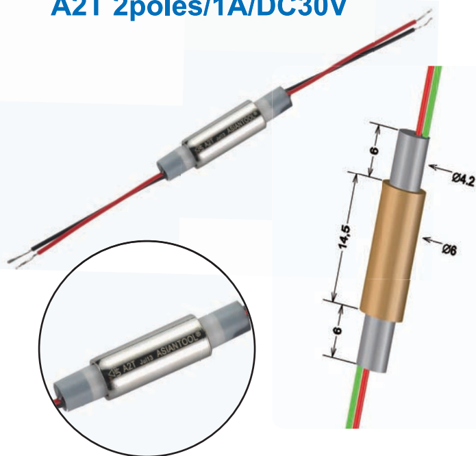
A2T 2poles/1A/DC30V
