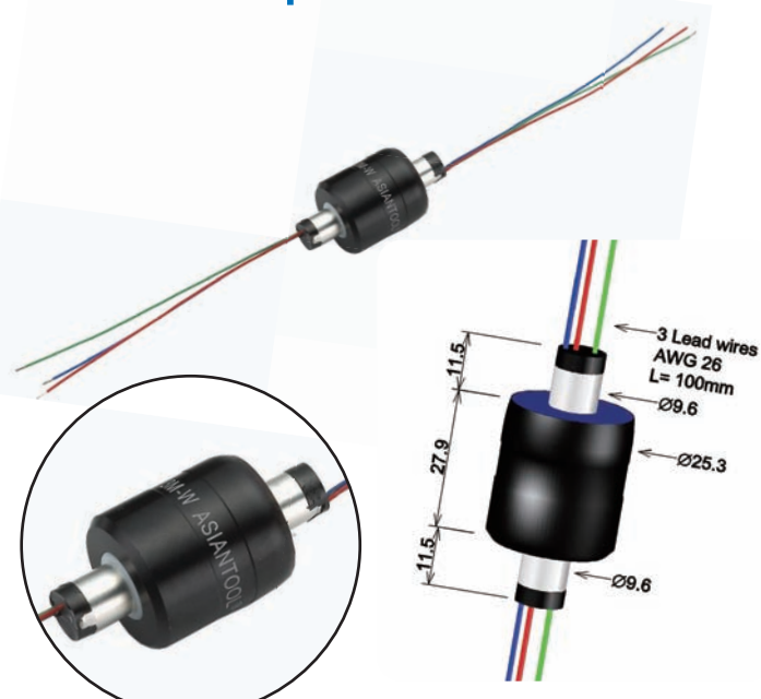
A3M-W 3poles/4A/AC250V
