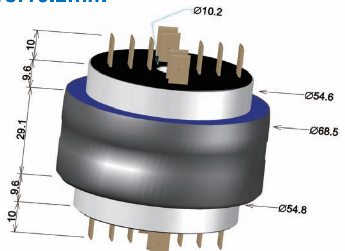
H103010NM (non-mercury) 10poles/30A/AC250V Through-bore:10.2mm
