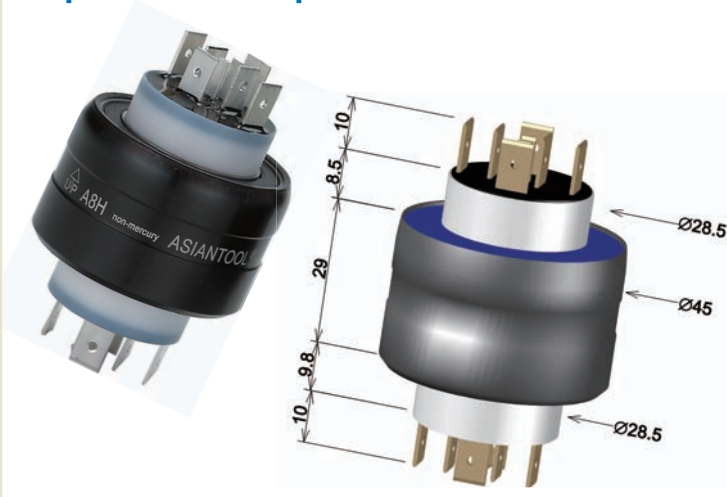
A8H NM (non-mercury) 6poles/30A & 2poles/4A AC250V
