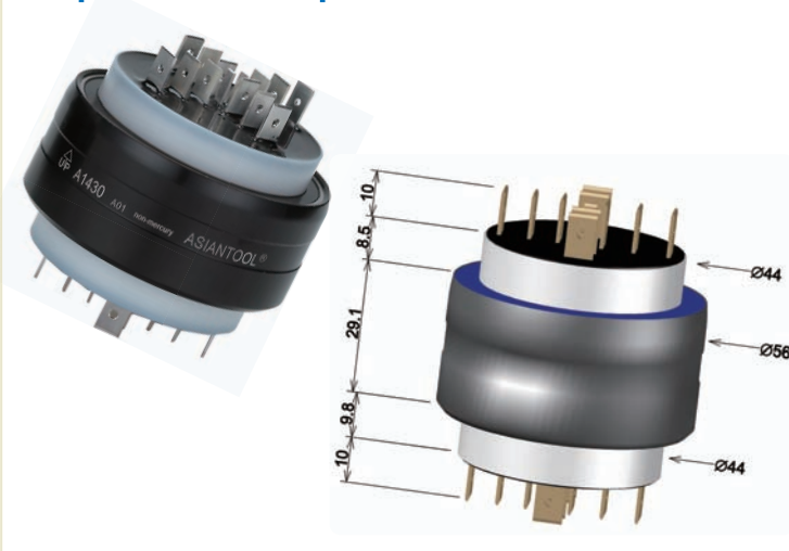
A1230 NM (non-mercury) 10poles/30A & 2poles/4A AC250V
