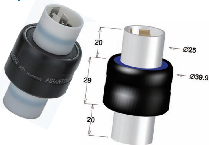
A3HV NM (non-mercury) 3poles/30A/AC500V
