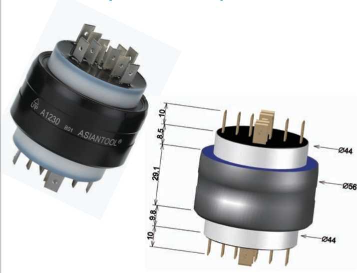
A1230 10poles/30A & 2poles/4A AC250V
