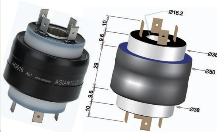
H43016 NM (non-mercury) 4poles/30A/AC250V Through-bore:16.2mm
