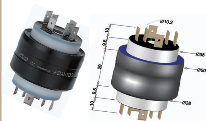
H63010 NM (non-mercury) 6poles/30A/AC250V Through-bore:10.2mm
