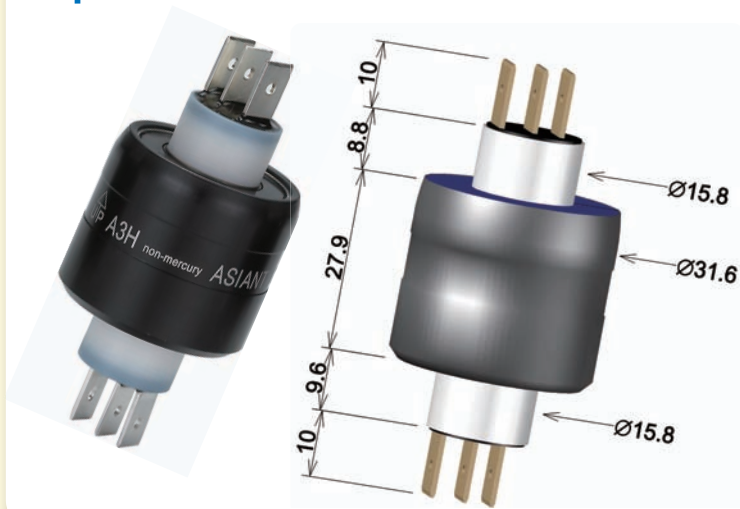
A3H NM (non-mercury) 3poles/30A/AC250V
