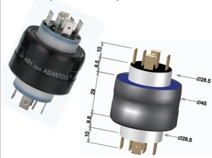
A8H 6poles/30A & 2poles/4A AC250V
