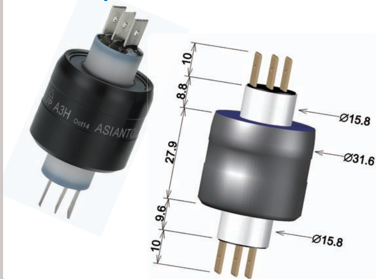
A3H 3poles/30A/AC250V
