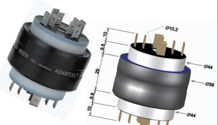
H83010 NM (non-mercury) 8poles/30A/AC250V Through-bore:10.2mm
