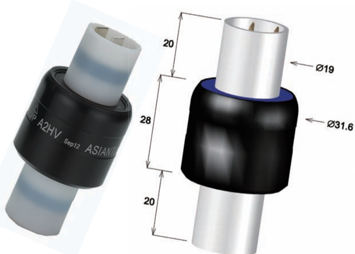
A2HV 2poles/30A/AC500V
