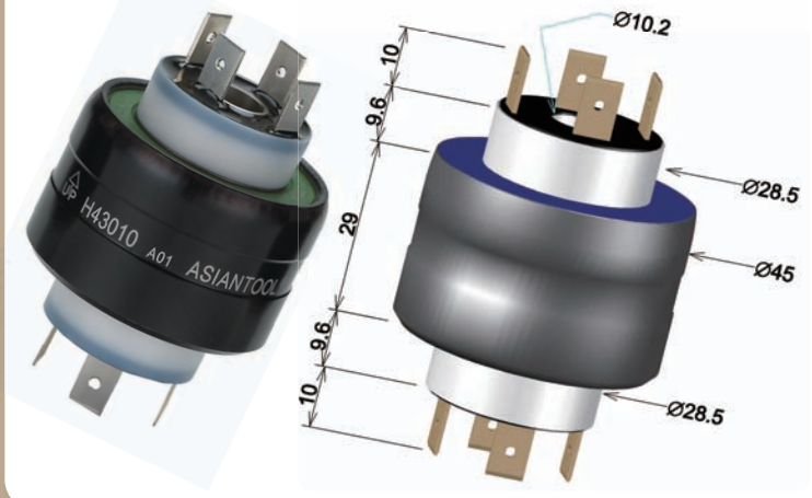
H43010 NM (non-mercury) 4poles/30A/AC250V Through-bore:10.2mm
